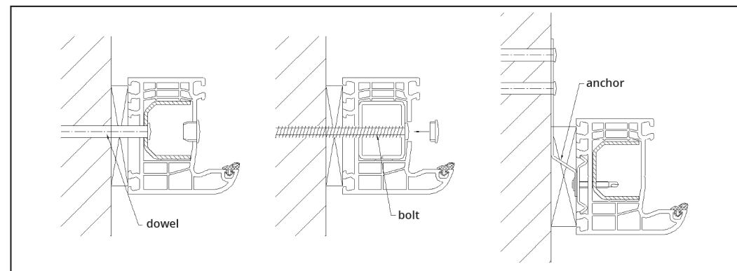
Fig. 6 Types of mechanic connectors.
