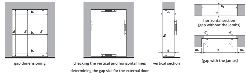
Fig. 2 Dimensioning the reveal in the wall: with and without the jamb.
