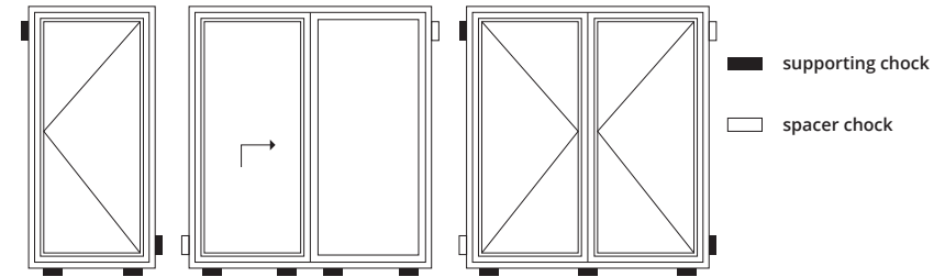
Fig. 1 The position of spacer chocks to determine the woodwork position.
